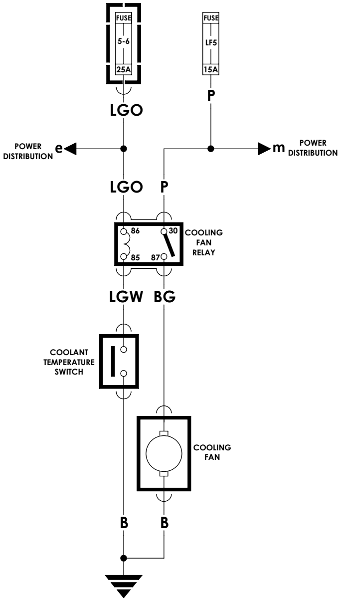
AUXILIARY COOLING FAN CIRCUIT 86M2576
