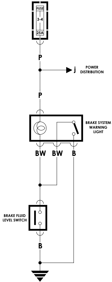
BRAKE TEST CIRCUIT 86M2579
