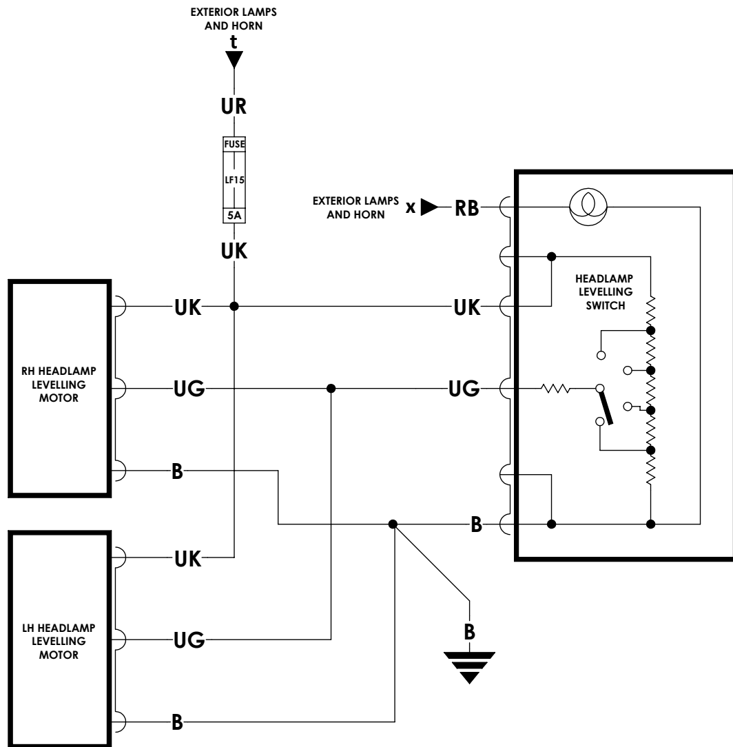
HEADLAMP LEVELLING CIRCUIT
