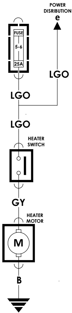
HEATER CIRCUIT 86M2571
