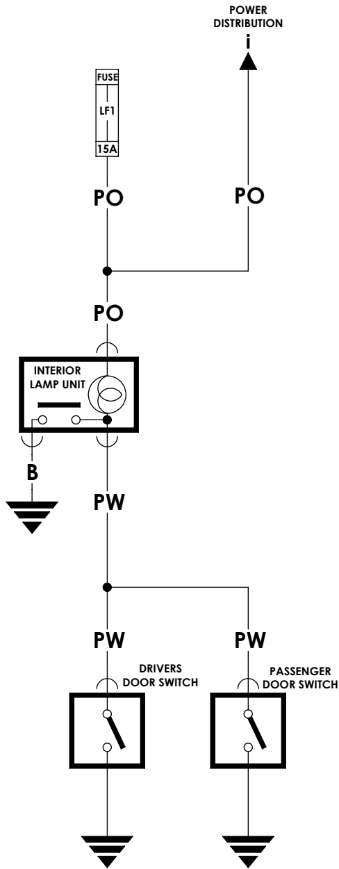
INTERIOR LAMP CIRCUIT (SALOON) 86M2569
