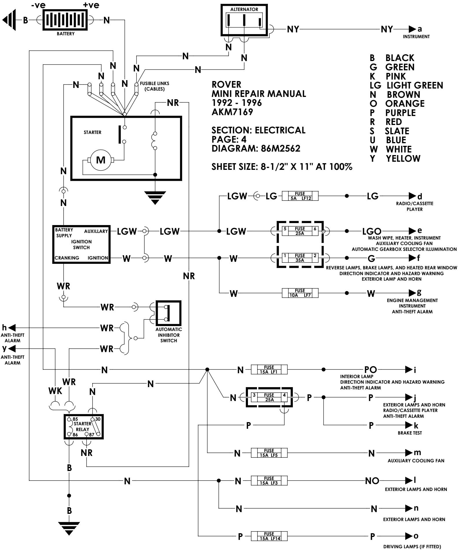
POWER DISTRIBUTION - CABURETTER MODELS
