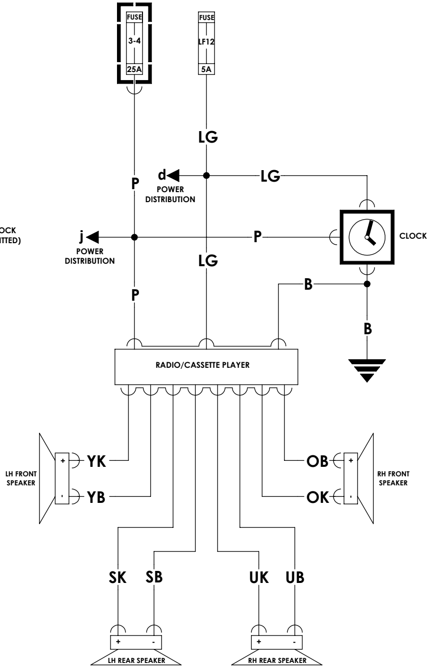
RADIO/CASSETTE PLAYER 4 SPEAKER SYSTEM 86M2578
