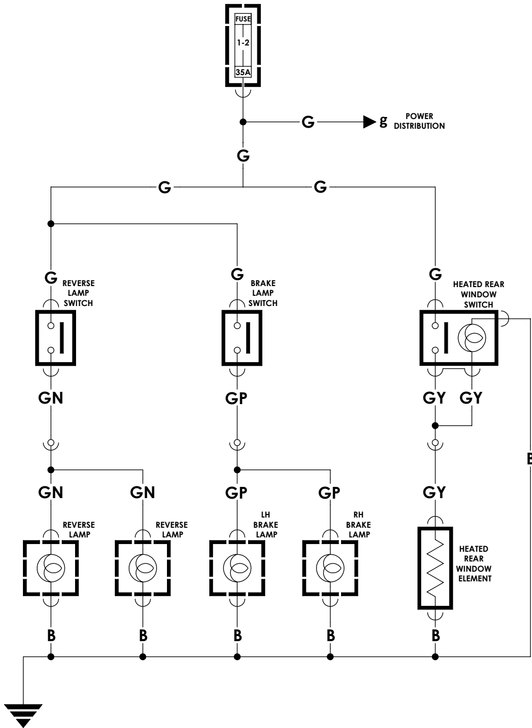
REVERSE LAMPS, BRAKE LAMPS AND HEATED REAR WINDOW CIRCUIT
